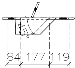
Cleat & Notch Dimensions
