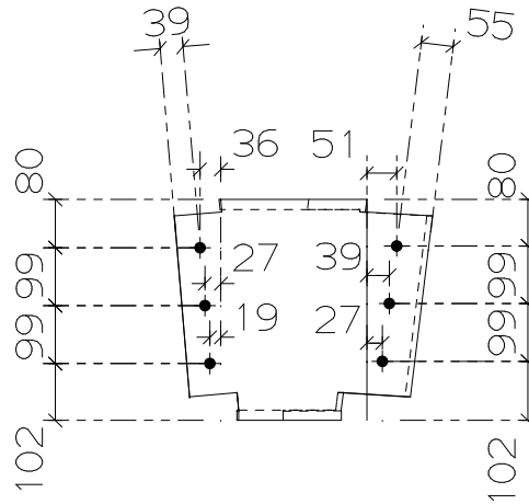
Hole Dimensions
